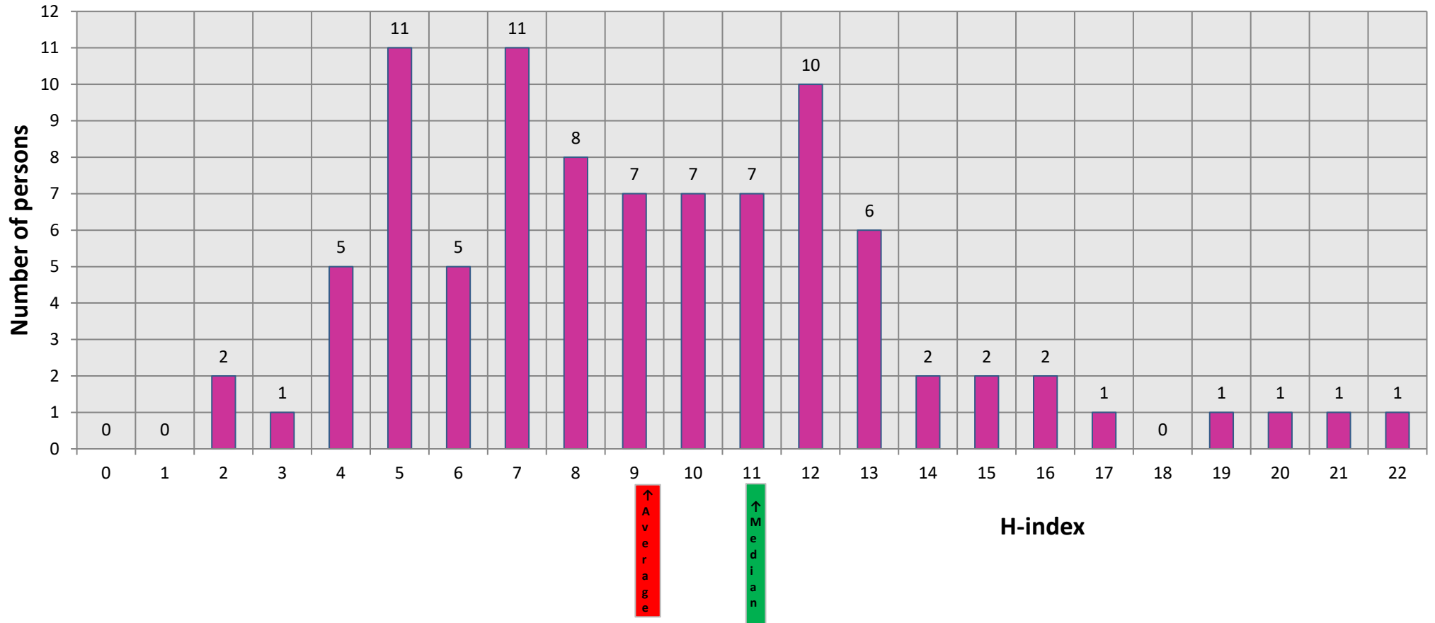
Hirsch Index for TE2023 Project Leaders
