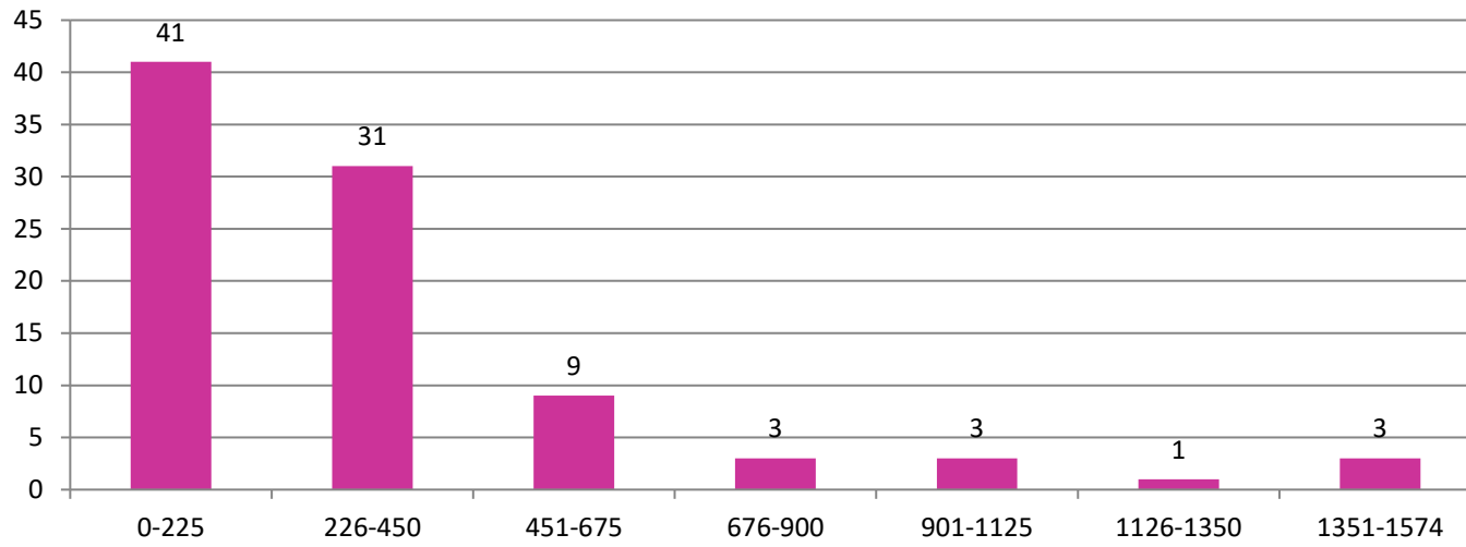
Distribution of TE2023 Project Leaders by citation groups
