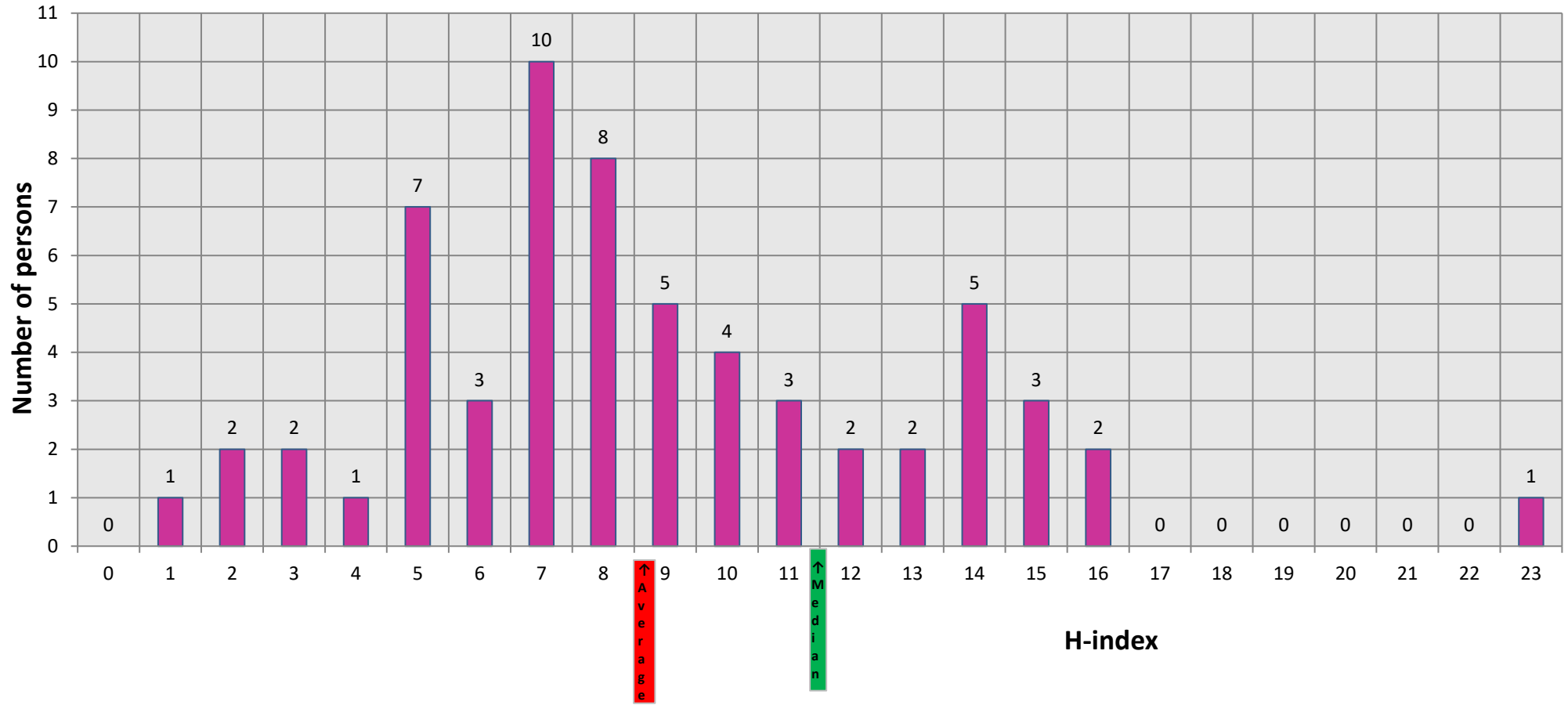
Hirsch Index for TE2023 Project Leaders
