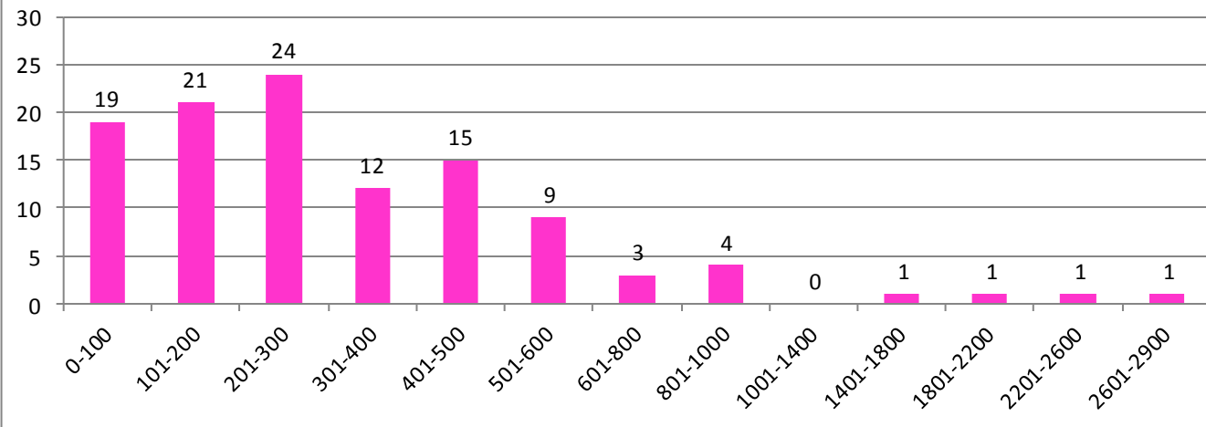
Distribution of TE 2021 directors by citation groups
