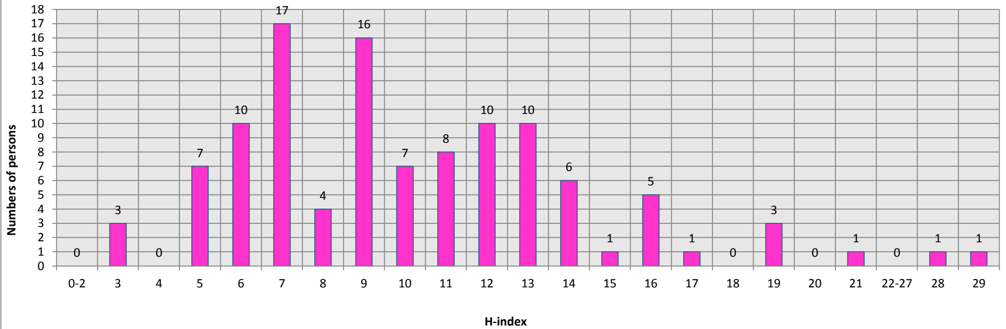
H-index for TE 2021 project leaders
